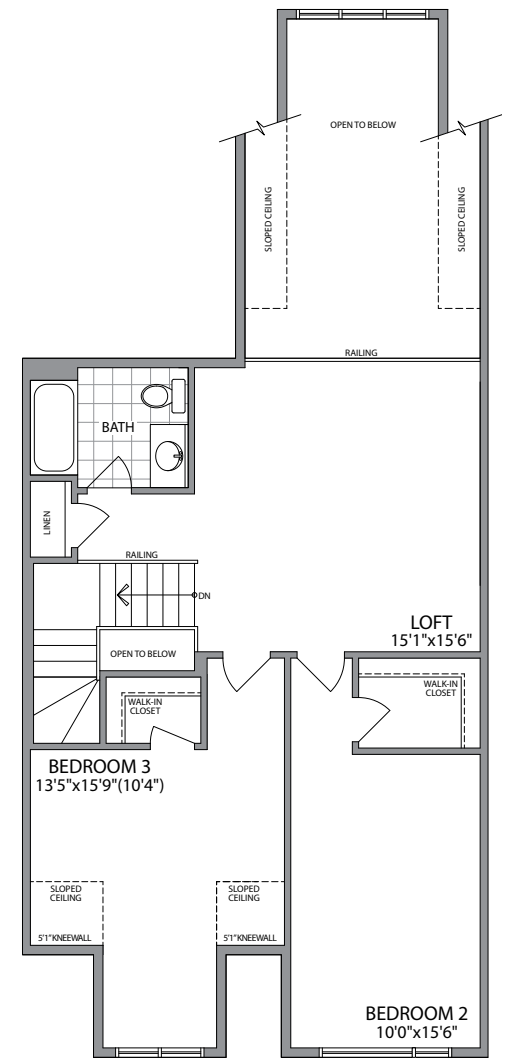
LOFT ELEVATION B
