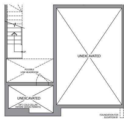
BASEMENT ELEVATION B & B1
