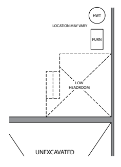
BASEMENT FOR SUNKEN MUDROOM (2R-3R) ELEV. A, A1, B & B1
