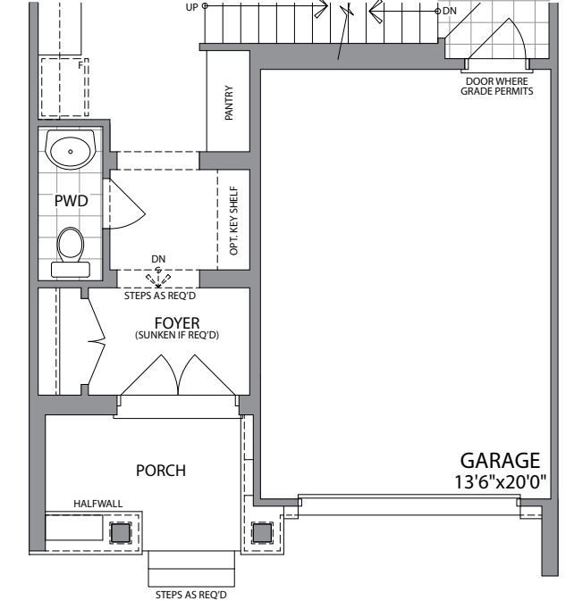
GROUND FLOOR ELEVATION A1
