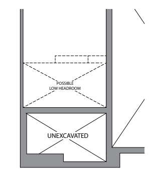
BASEMENT FOR SUNKEN FOYER (2R) ELEV. A, A1, B & B1
