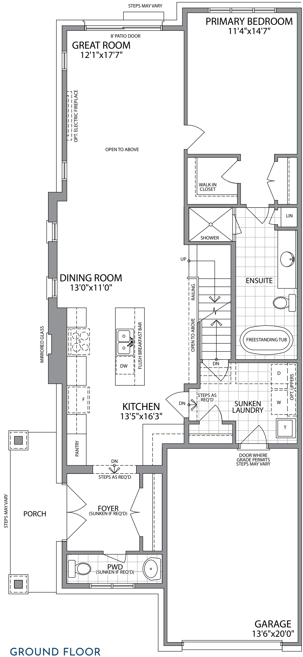
GROUND FLOOR ELEVATION A
