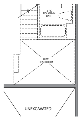
BASEMENT FOR SUNKEN LAUNDRY (2R) ELEV. A & B
