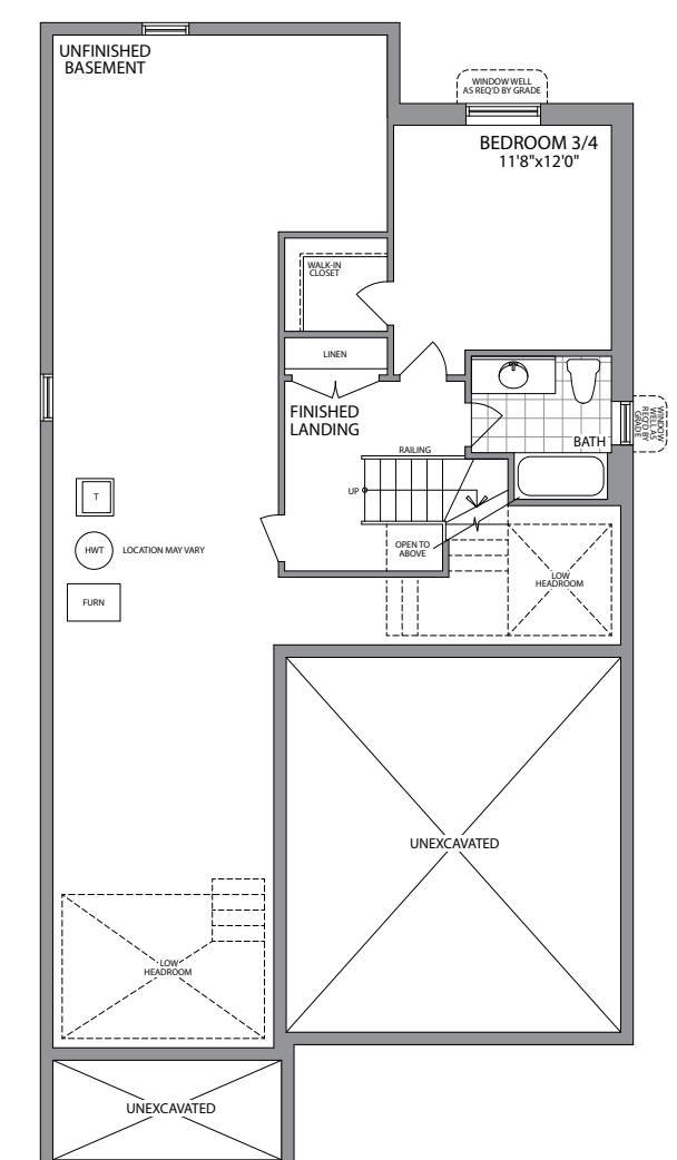
BASEMENT ELEVATION A & A1
