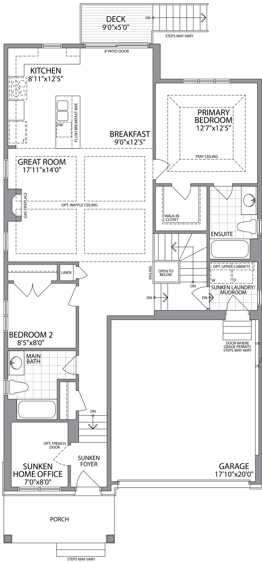
GROUND FLOOR ELEVATION A
