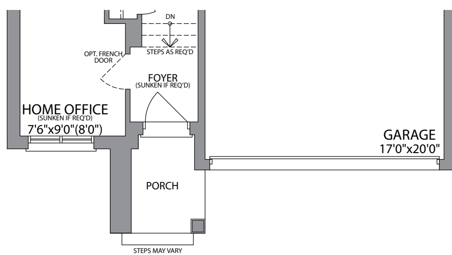
GROUND FLOOR ELEVATION B
