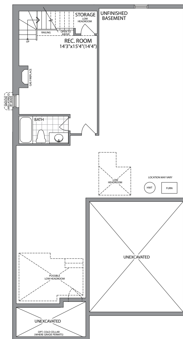
BASEMENT ELEVATION B
