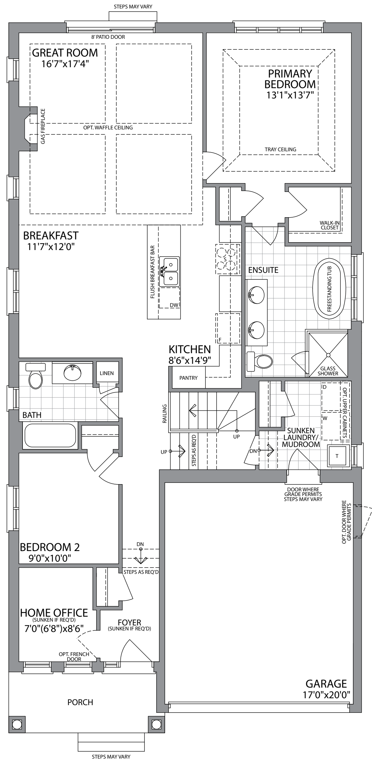
GROUND FLOOR ELEVATION A1
