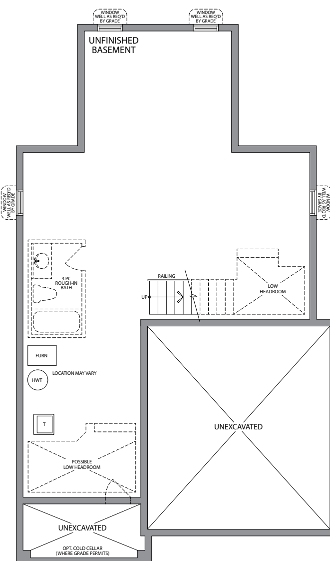
BASEMENT ELEVATION A & A1
